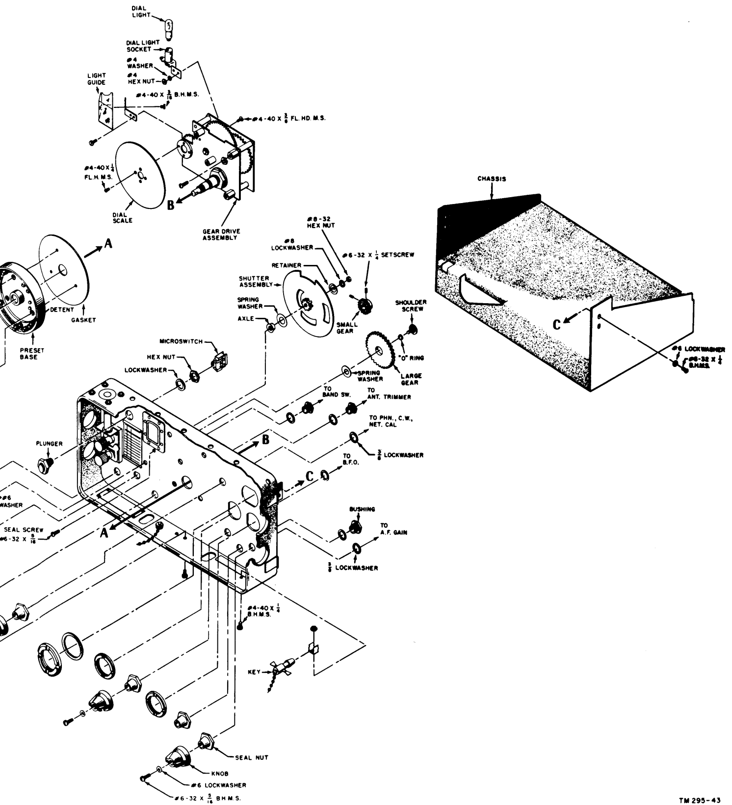
Receiver R-174/URR, front panel assembly, exploded view.
