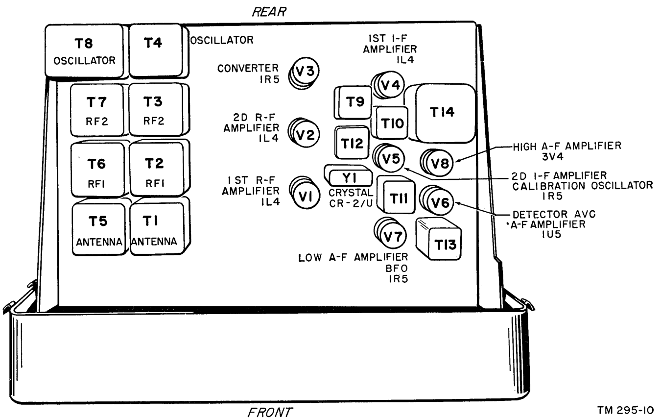
Figure 6. Radio Receiver R-174/URR, tube location.
