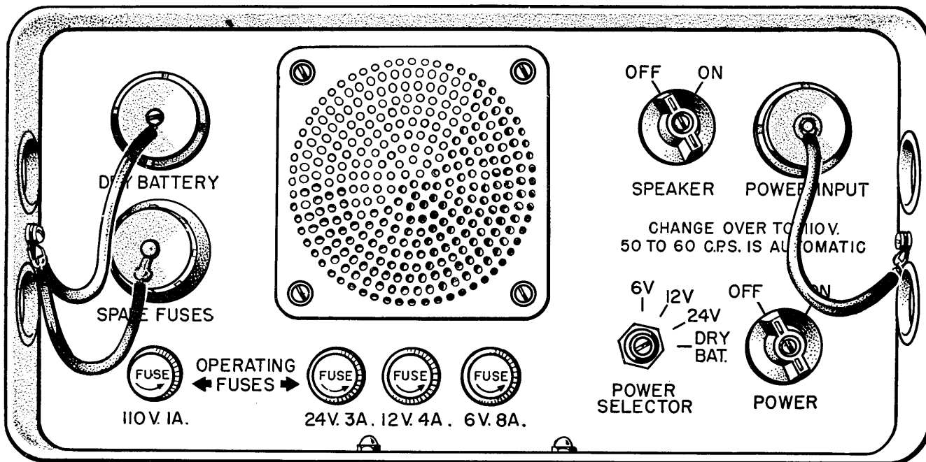
Figure 13. Power Supply PP-308/URR, front panel.
